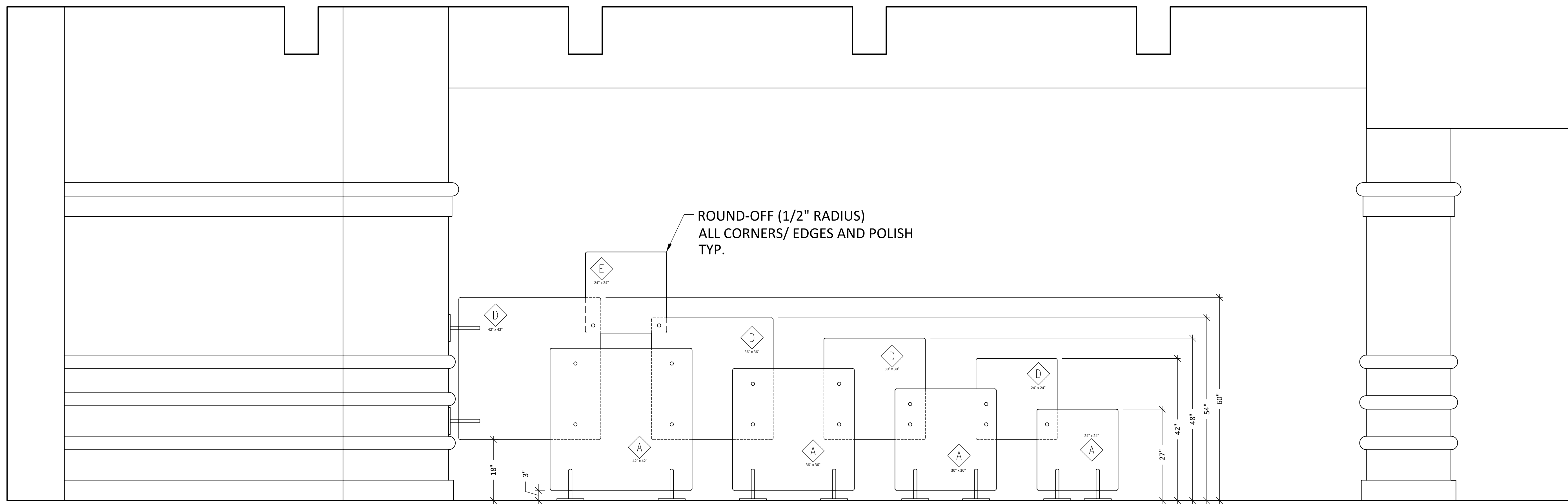
A ELEVATION-3 FORM SCREENS Scale: 3/4" = 12"
