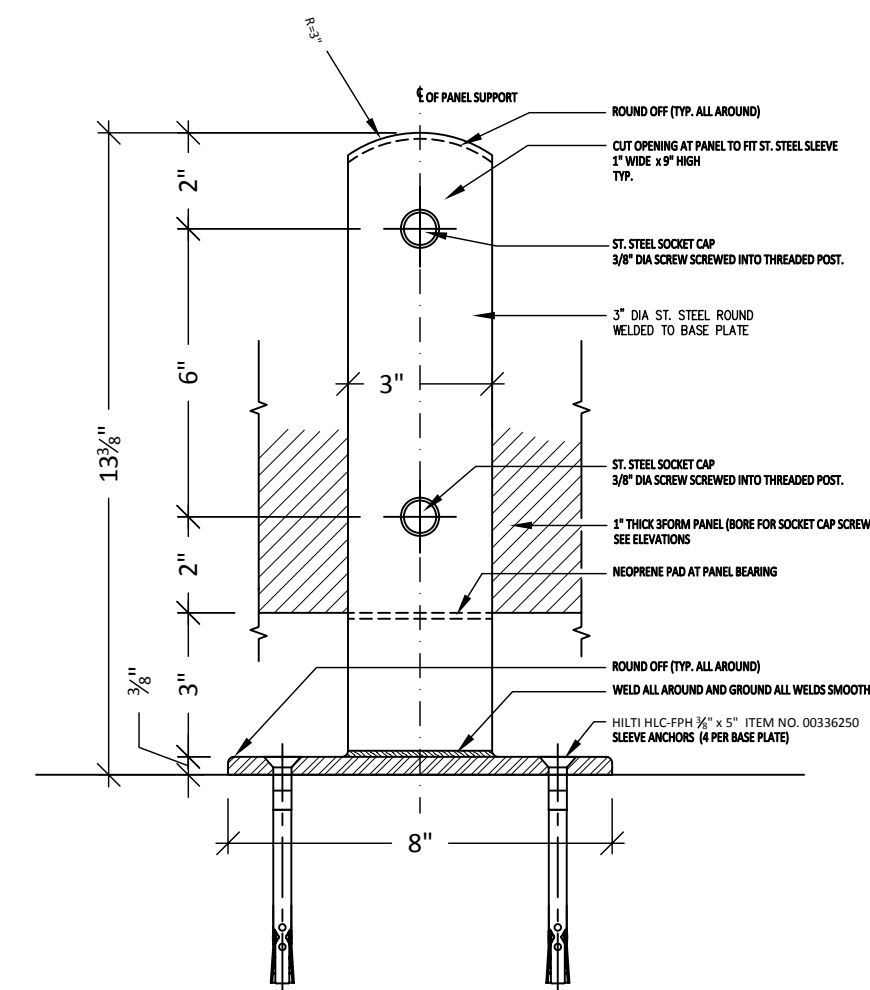
D.2 DETAIL- @ PANEL SUPPORT Scale: 3" = 12"
