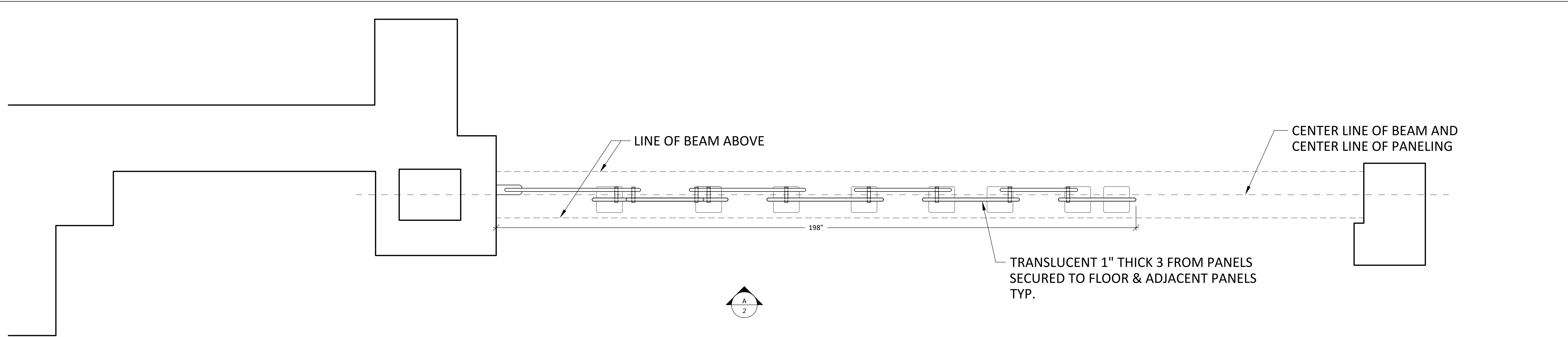
1 PLAN VIEW- 3 FORM SCREENS Scale: 3/4" = 12"
