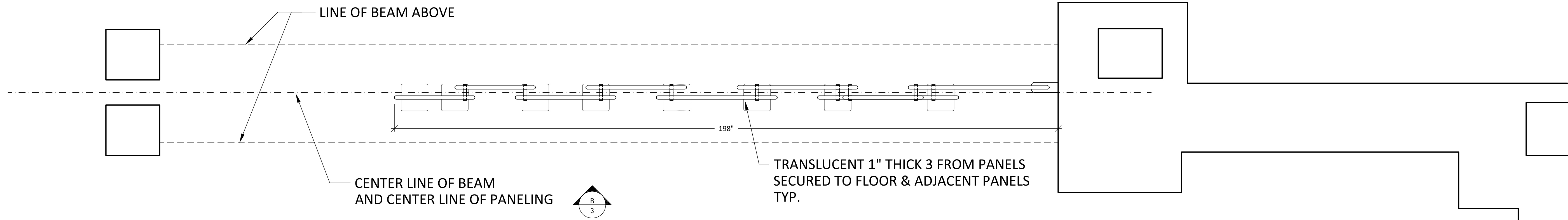
2 PLAN VIEW -3 FORM SCREENS Scale: 3/4" = 12"
